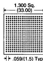
Footprint 361
