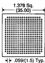
Footprint 396
