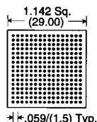
Footprint 256-5
