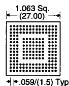
Footprint 193
