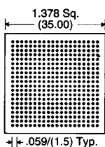
Footprint 400-1
