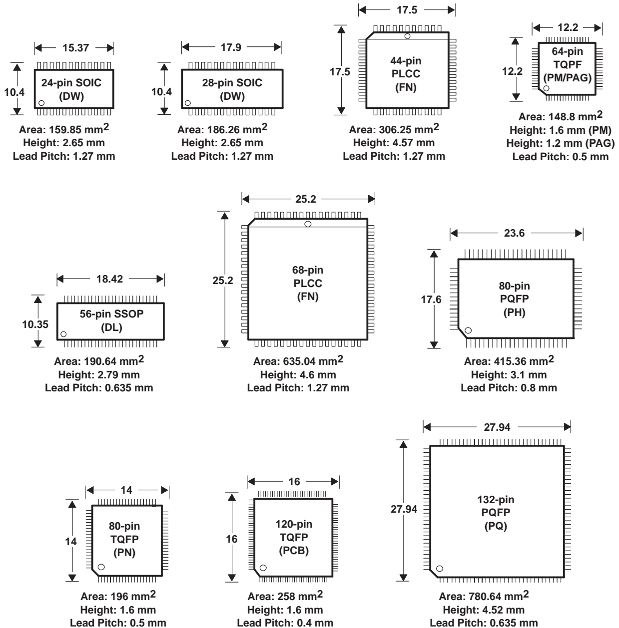
Figure 1. Package Dimensions
